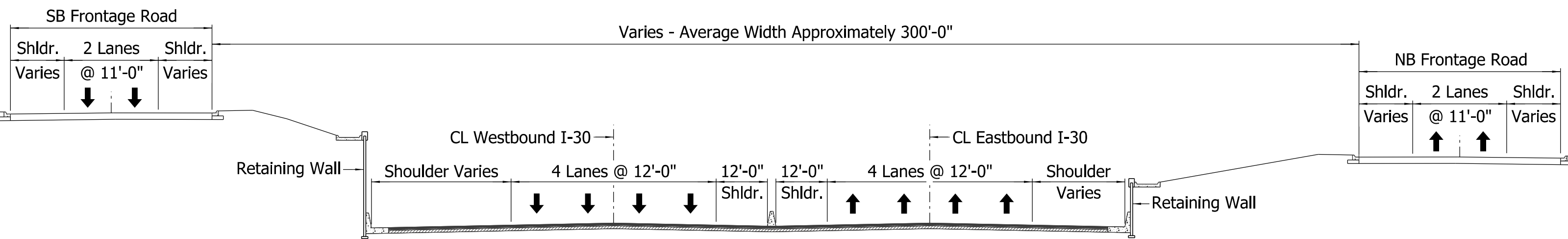
TYPICAL SECTION (I-30 & FRONTAGE ROADS)
