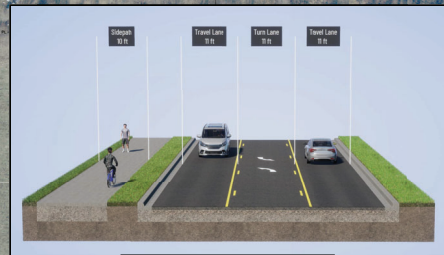
TYPICAL SECTION E. KENWOOD STREET
